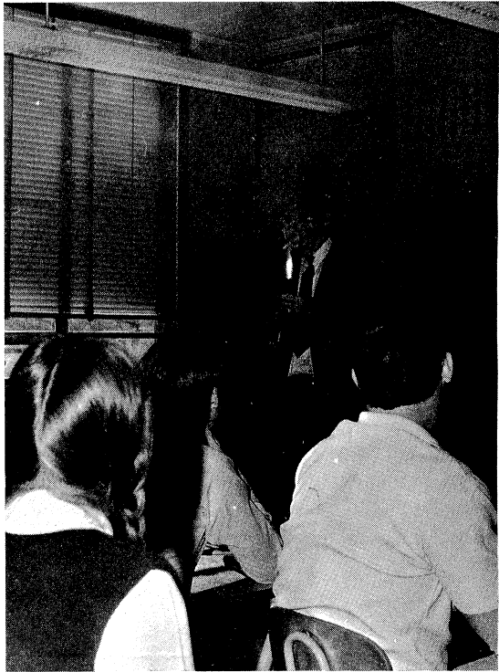
In the presence of attentive students, Mr. Coates burns some magnesium for his chemistry class.
